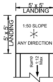
ACCESSIBLE RAMP LANDING
