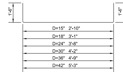
BENDING FOR V2 - BARS
