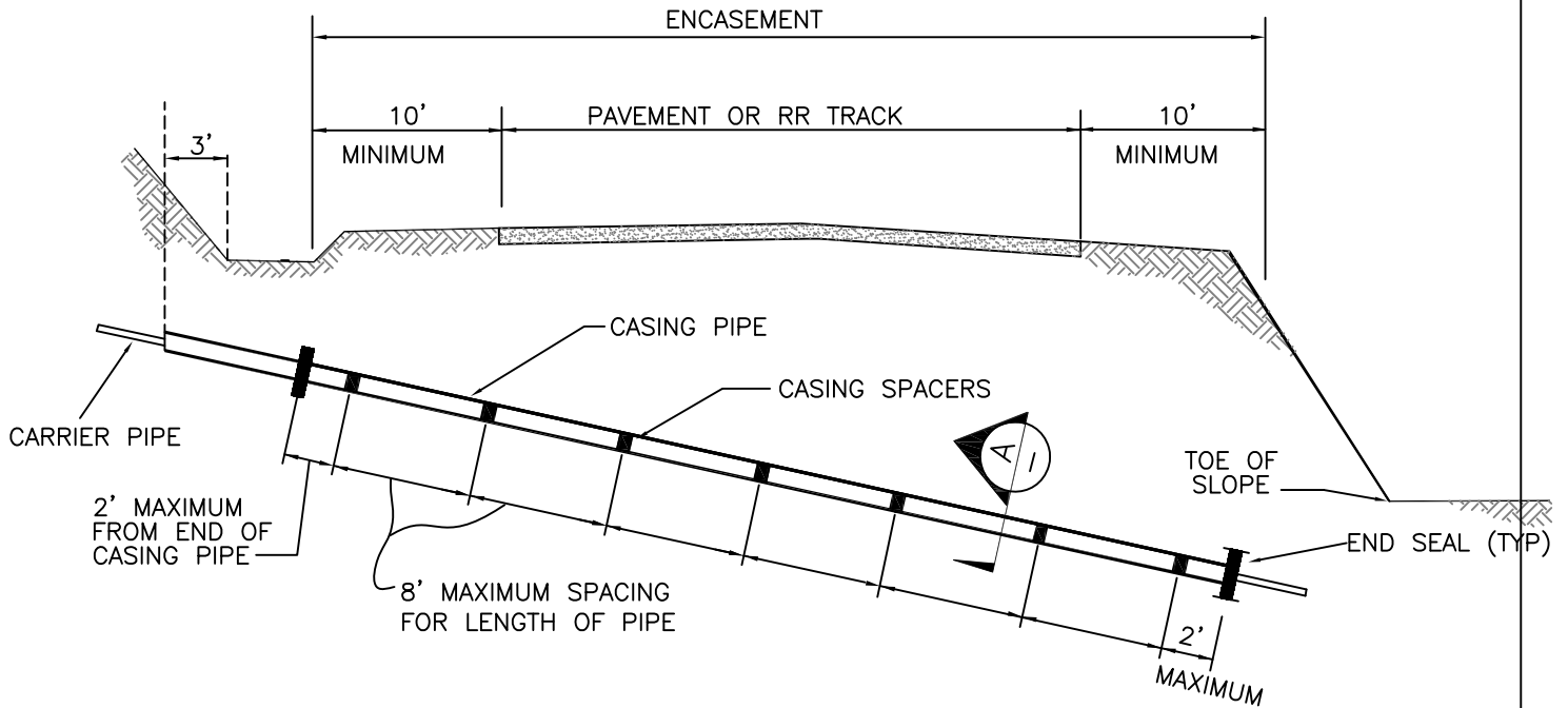
ROAD SECTION
