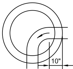
TYPICAL MANHOLE INVERT DETAIL
