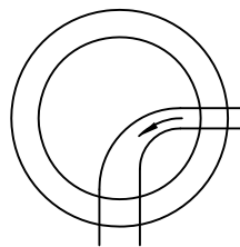
TYPICAL MANHOLE INVERT DETAIL
