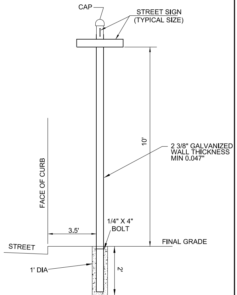
STREET SIGN DETAIL CONCRETE BASE
